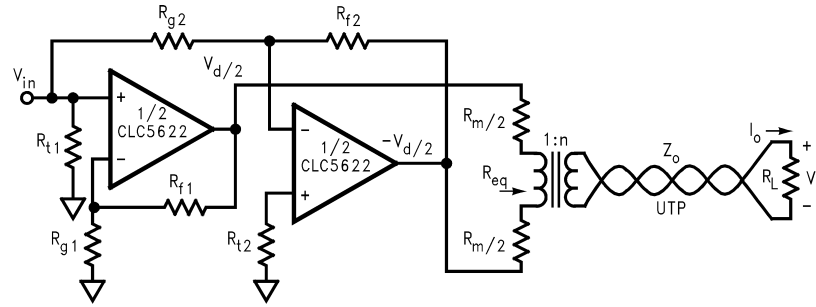
Differential Line Driver with Load Impedance Conversion
