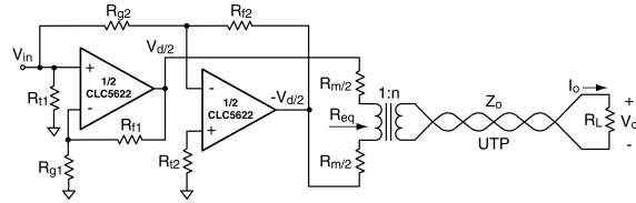
FIGURE 15. Differential Line Driver with Load Impedance Conversion
