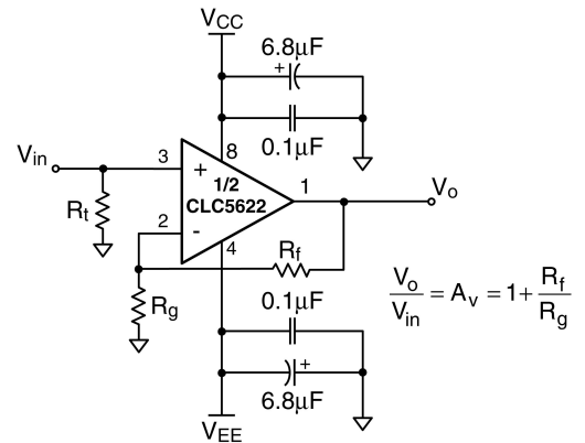
FIGURE 5. Dual Supply Non-Inverting Configuration
