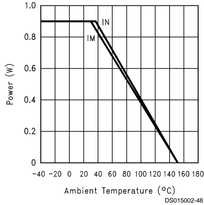
FIGURE 9. Power Derating Curves
