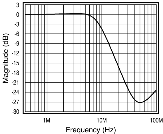
FIGURE 14. Lowpass Response
