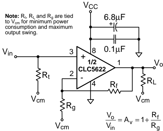
FIGURE 1. Non-Inverting Configuration
