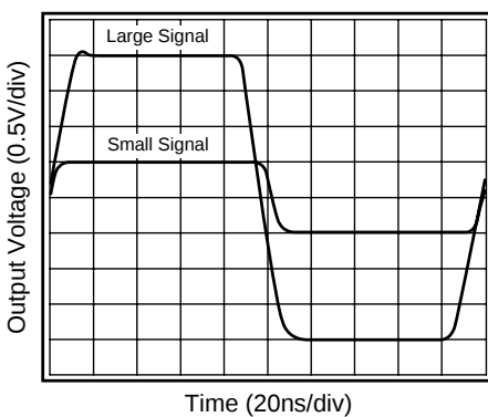
Large &amp; Small Signal Pulse Response
