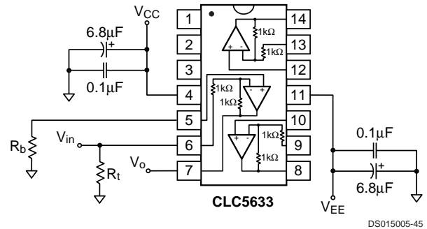
FIGURE 7. Dual Supply, A_V = -1/V_V Configuration
