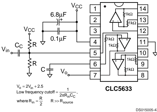
FIGURE 5. AC Coupled, A_V = +1/V_V Configuration
