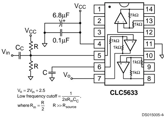
FIGURE 6. AC Coupled, A_V = +2/V_V Configuration
