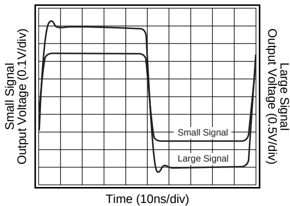
Large & Small Signal Pulse Response
