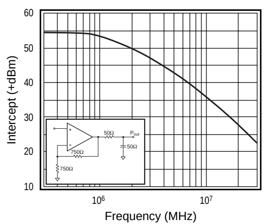
2-Tone, 3rd Order Intermodulation Intercept
