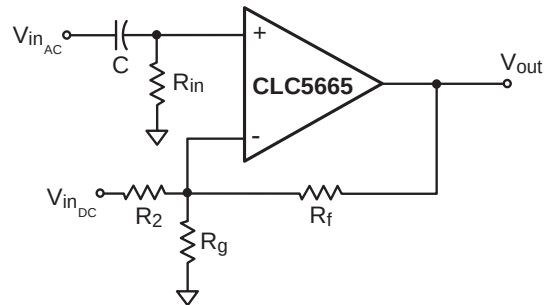
FIGURE 5. Level Shifting Circuit
