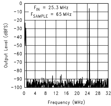
Spectral Response
