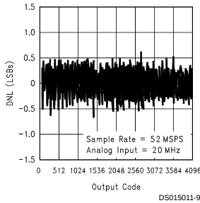
Differential Non-Linearity
