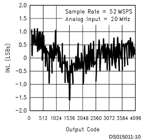
Integral Non-Linearity
