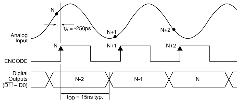
CLC952B Timing Diagram
