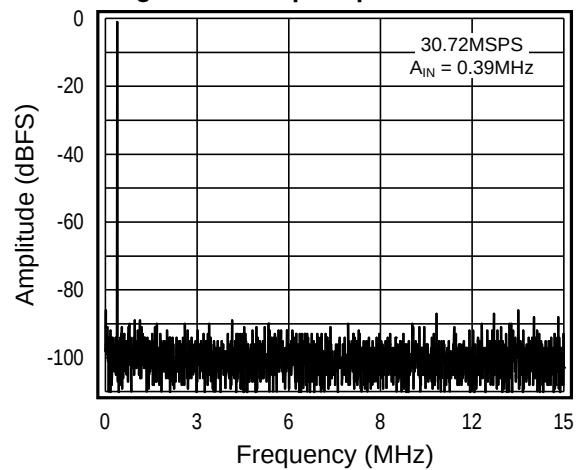
Single Tone Output Spectrum
