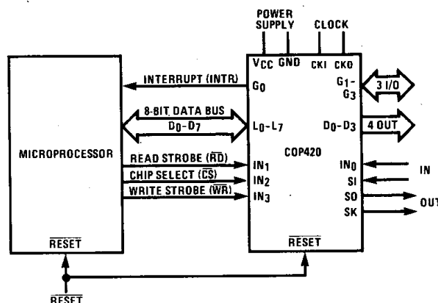
Figure 6. MICROBUS™ Option Interconnect
