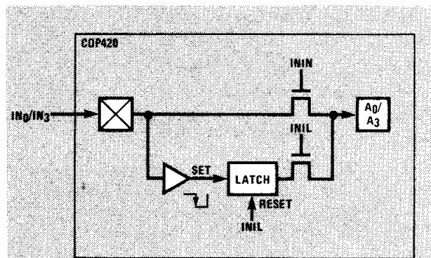
Figure 3.1 INIL Hardware Implementation
