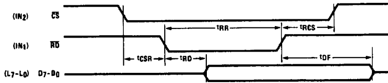
FIGURE 4. Microbus Read Operation Timing
