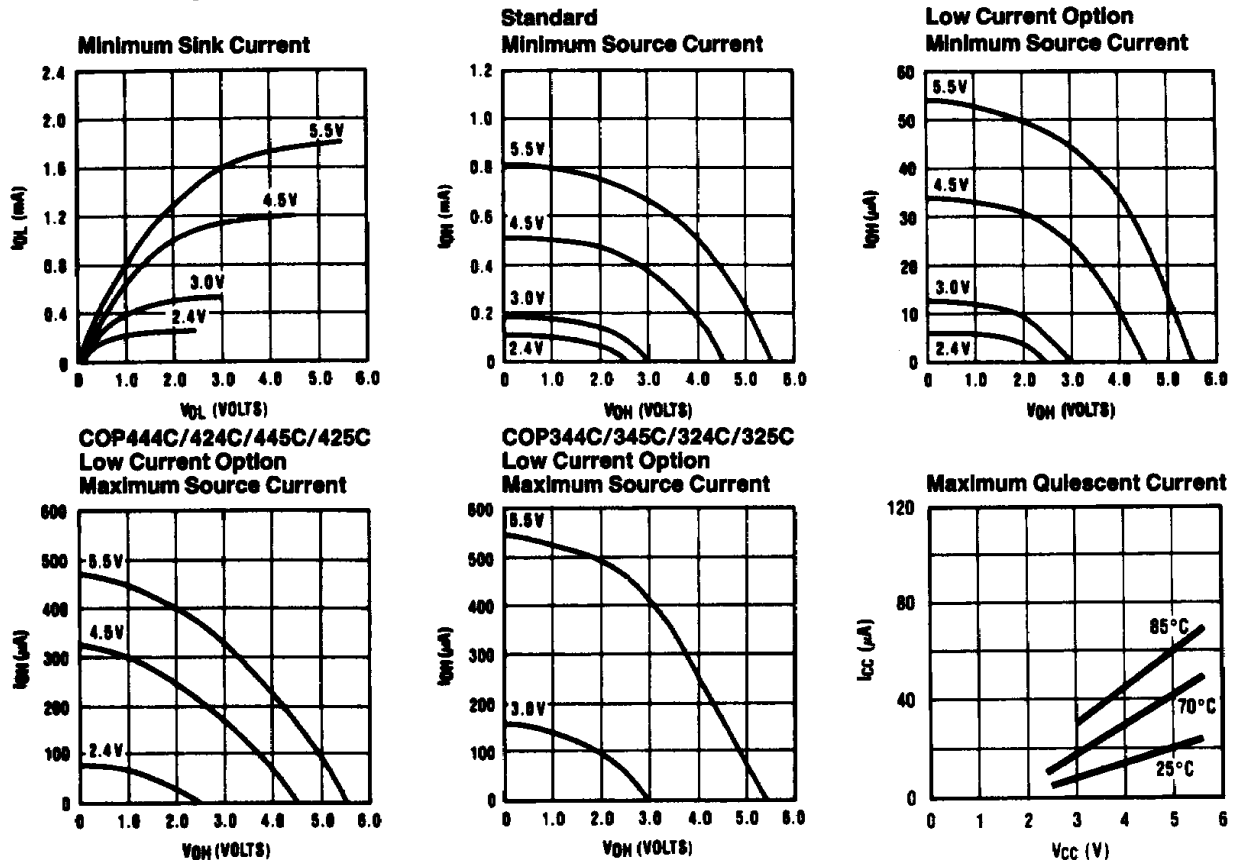
FIGURE 12. Input/Output Characteristics
