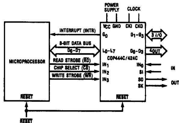
FIGURE 6. Microbus Option Interconnect
