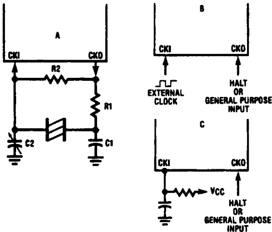
Crystal or Resonator
