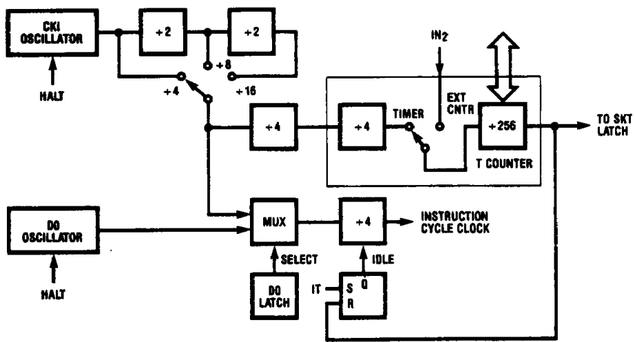
FIGURE 10B. Clock and Timer with Dual-Clock
