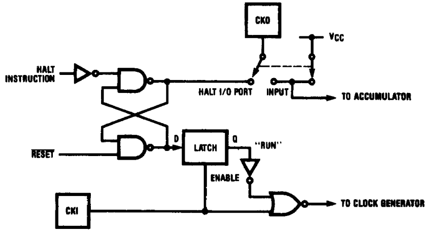
FIGURE 9B. Halt Mode — One-Pin Oscillator
