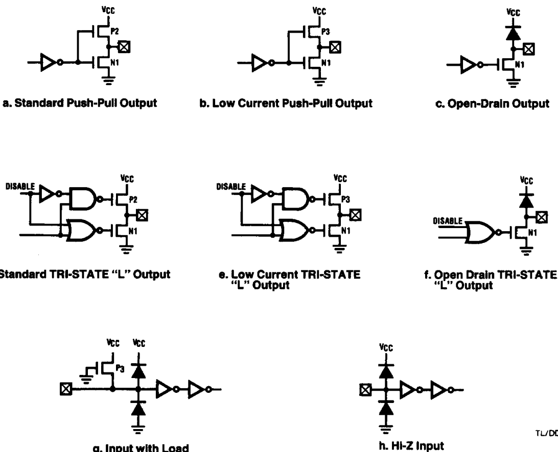
FIGURE 11. Input/Output Configurations
