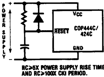
FIGURE 7. Power-Up Circuit
