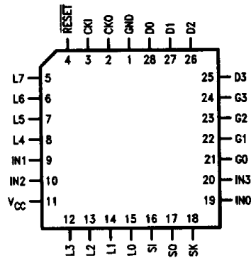
28 Lead PLCC
