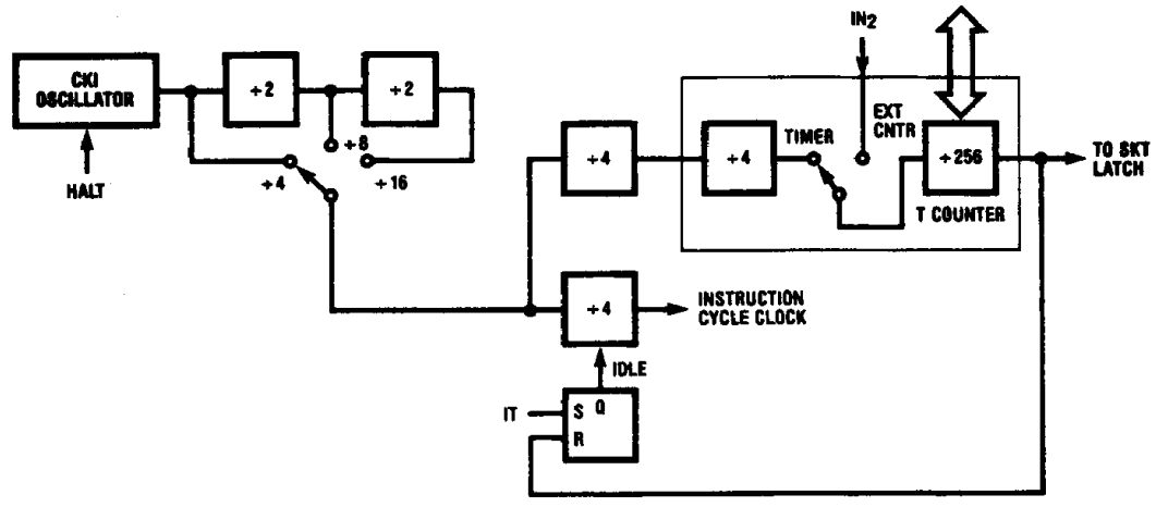
FIGURE 10A. Clock and Timer without Dual-Clock
