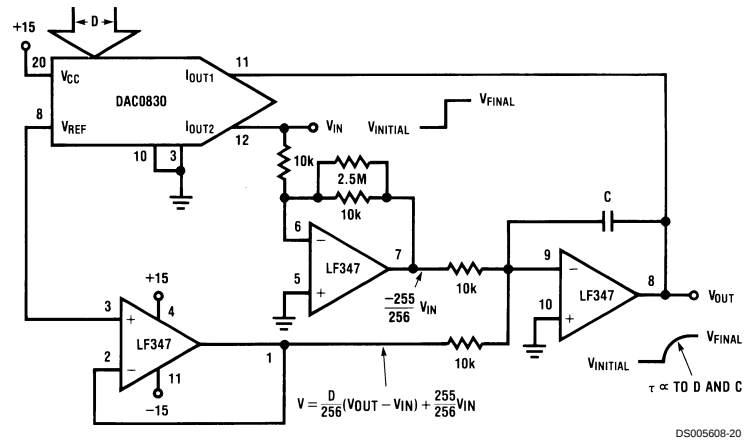
DAC Controlled Exponential Time Response
