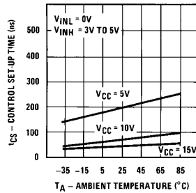
Control Set-Up Time, t_{CS}
