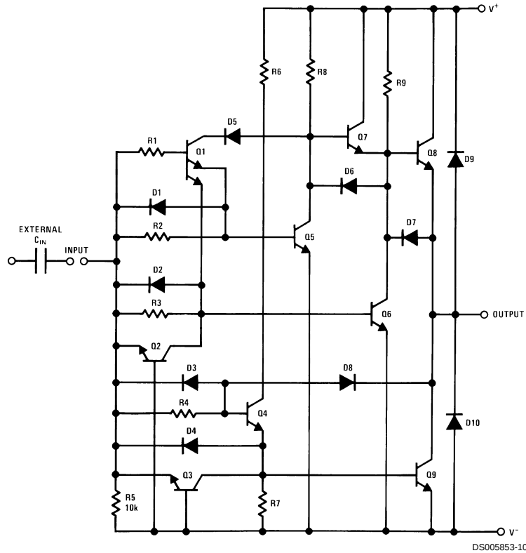
1/2 DS0026
