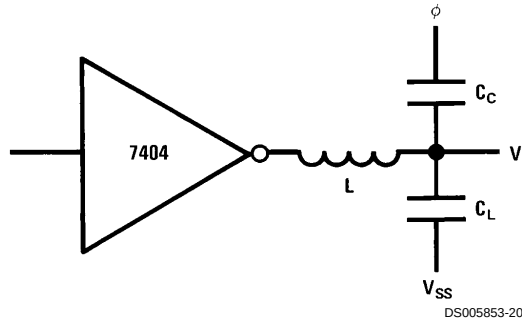
FIGURE 5. Clock Coupling
