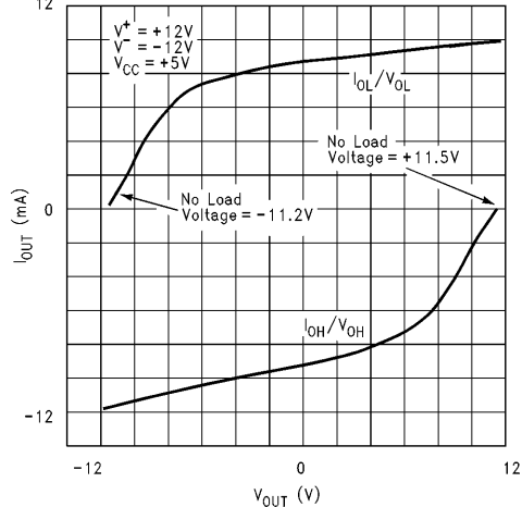
Driver Output Current vs Output Voltage
