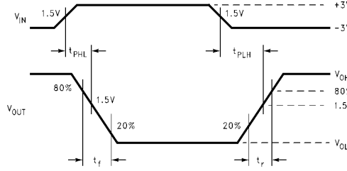
FIGURE 4. Receiver Propagation Delay and Transition Time Waveform
