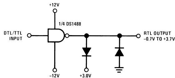
DTL/TTL-to-RTL Translator
