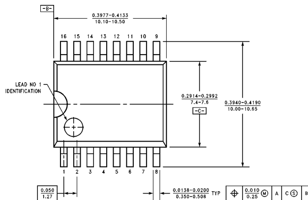
Order Number DS14C232CM or DS14C232TM NS Package Number M16
