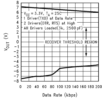
Driver Output vs Data Rate
