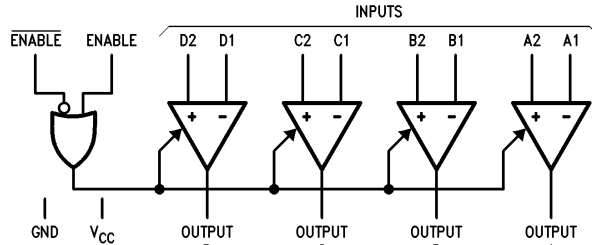
FIGURE 1. Logic Symbol
