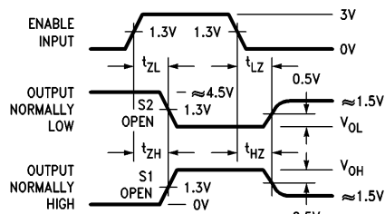
FIGURE 4. Enable and Disable Times (Notes 1, 2 and 3)
