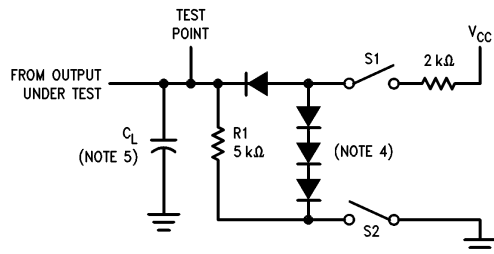
FIGURE 2. Load Test Circuit for Three-State Outputs
