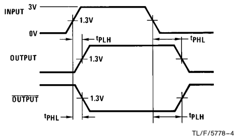
FIGURE 2. Propagation Delays
