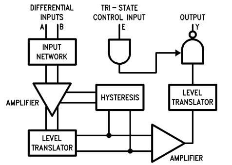
FIGURE 1. Block Diagram
