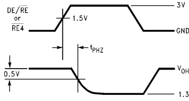
FIGURE 8. Receiver Enable and Disable Timing
