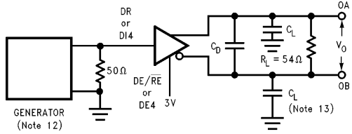
FIGURE 3. Driver Differential Propagation Delay Load Circuit
