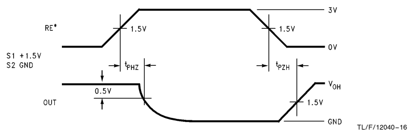
FIGURE 16. Receiver Enable and Disable Waveforms ( t_{PHZ} , t_{PZH} )
