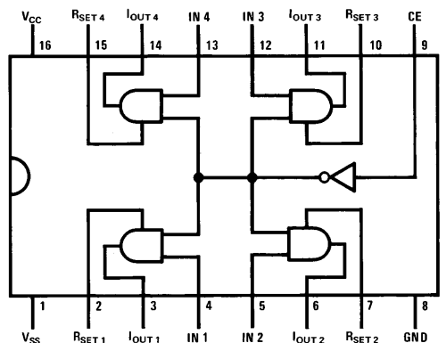
Dual-In-Line Package
