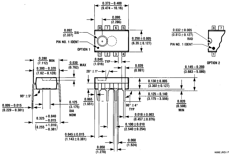
Molded Dual-In-Line Package (N) Order Number DS75150N NS Package Number N08E
