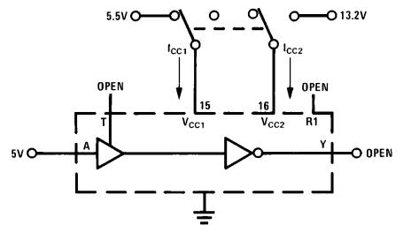
FIGURE 5. I_{CC}
