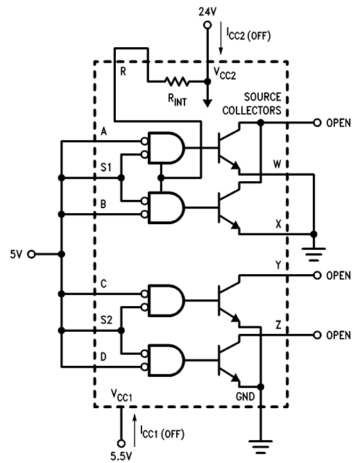
FIGURE 6. I_{CC1}(\text{OFF}) and I_{CC2}(\text{OFF})
