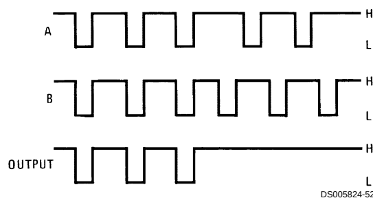
FIGURE 22. In-Phase Detector
