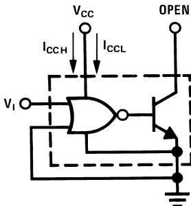
FIGURE 11. I CCH , I CCL for OR, NOR Circuits
