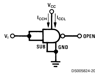
FIGURE 6. I_{CCH} , I_{CCL}
