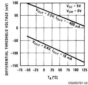
Temperature Sensitivity
