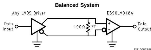
FIGURE 3. Point-to-Point Application
