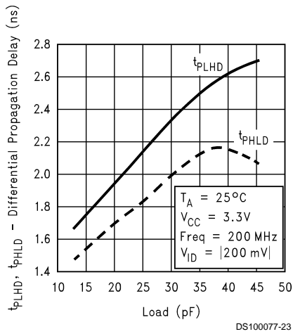
Differential Propagation Delay vs Load
