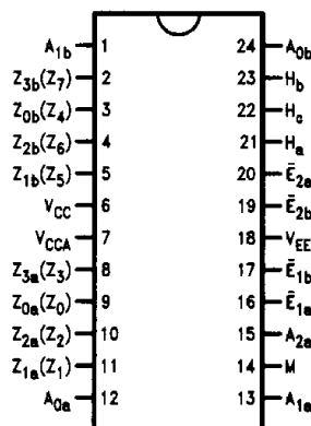
24-Pin DIP
