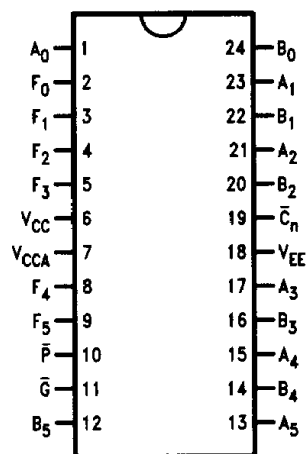
24-Pin DIP
