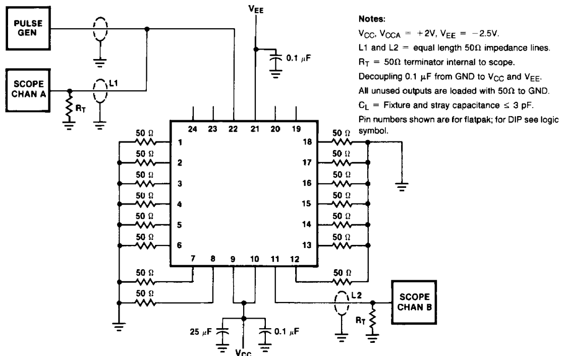
FIGURE 1. AC Test Circuit
