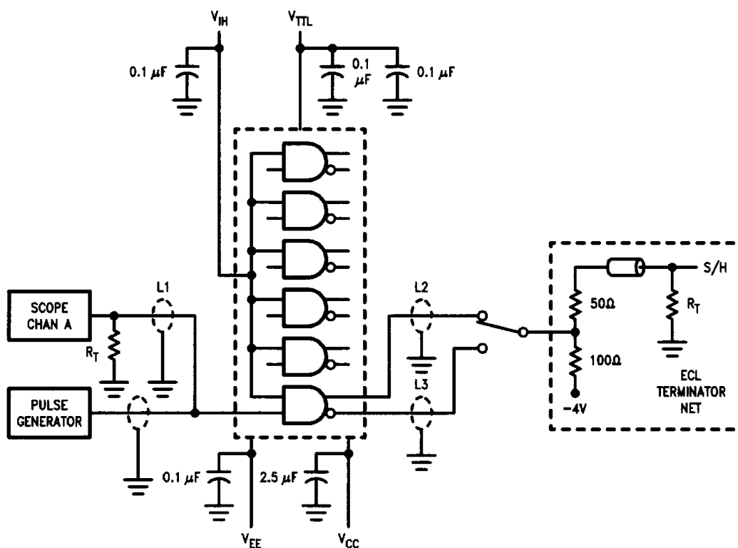
FIGURE 2. AC Test Circuit
