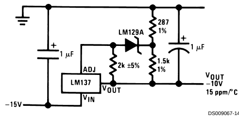
High Stability -10V Regulator
