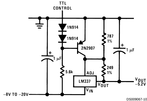
-5.2V Regulator with Electronic Shutdown*
