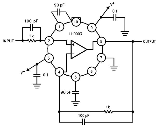
Unity Gain Follower
