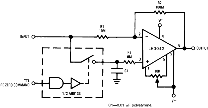
Re-Zeroing Amplifier
