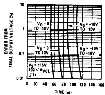
FIGURE 14. Settling Time
