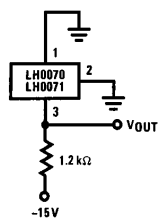
Negative 10V Reference
