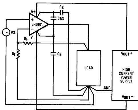
FIGURE 1. Single-Point Grounding
