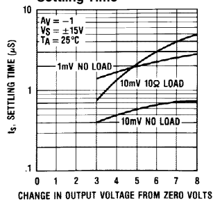
Settling Time
