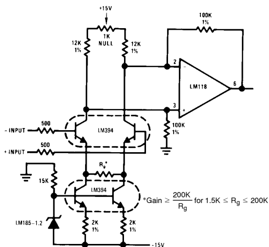
Instrumentation Amplifier
