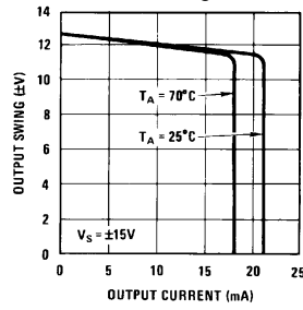
Current Limiting
