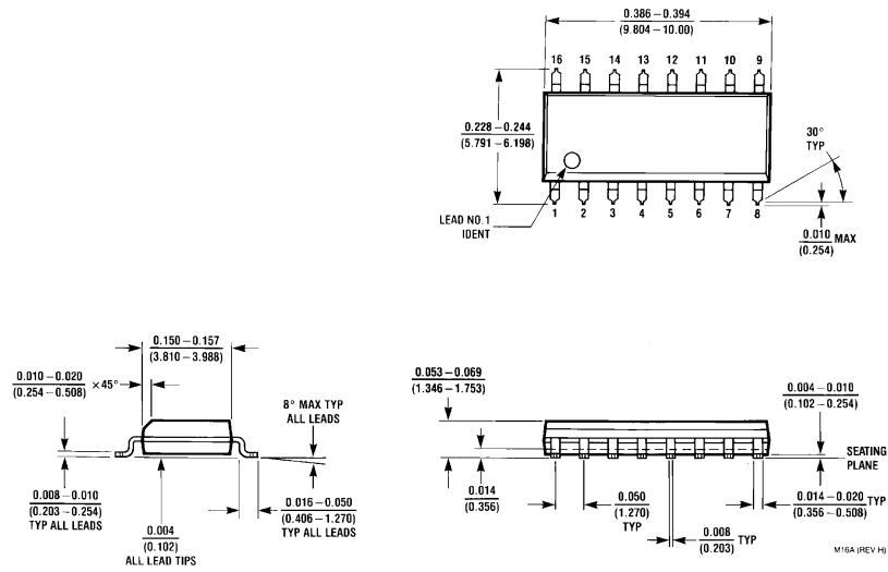
16-Lead (0.1500" Wide) Small Outline Molded Package (M) Order Number LM1201M NS Package Number M16A
