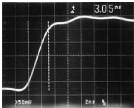
FIGURE 17c. LM1209 Rise Time
