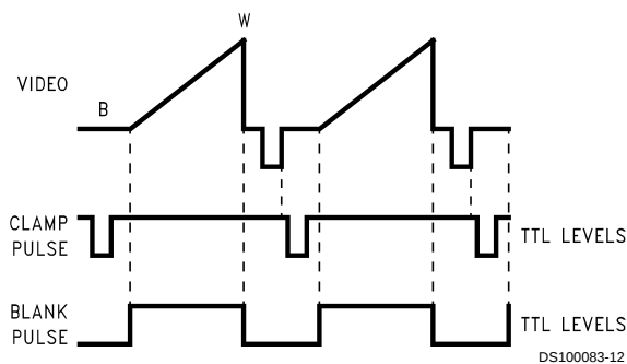
FIGURE 7. Timing Diagram
