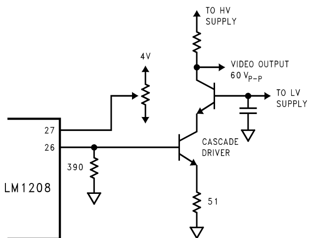
FIGURE 19. LM1208 Typical Application
