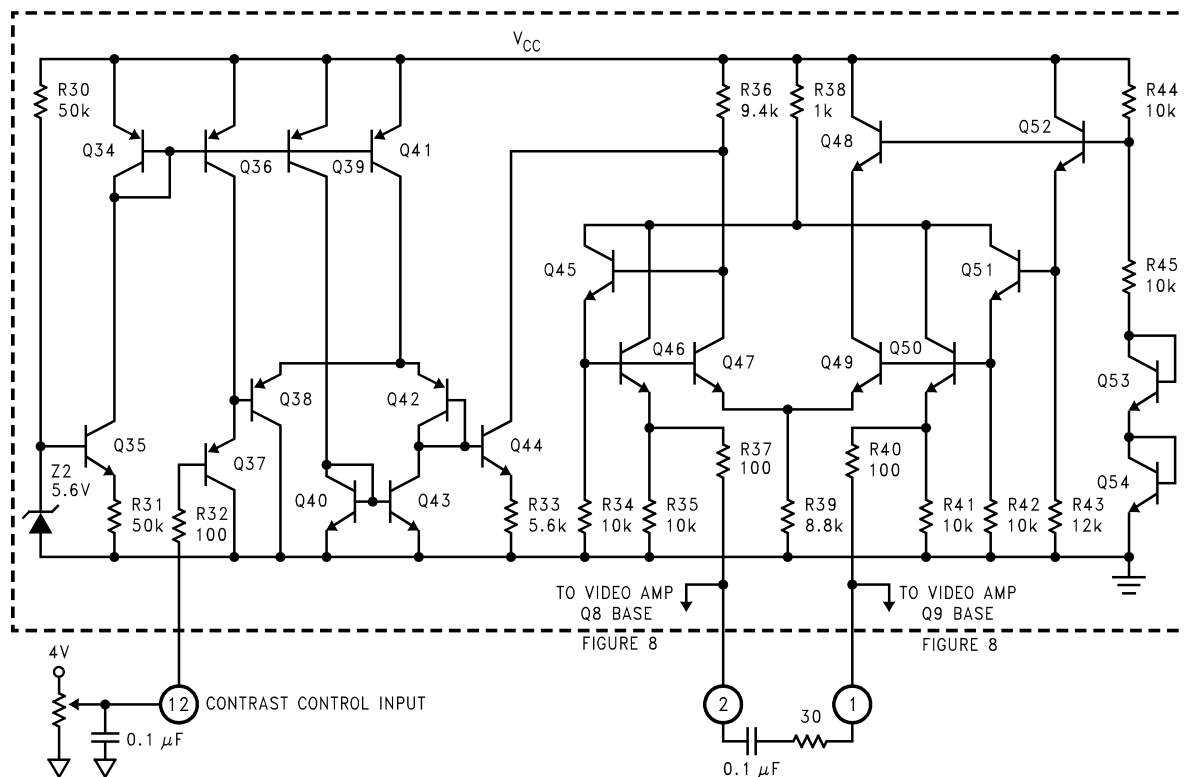
FIGURE 9. Simplified Schematic of LM1208 Contrast Control
