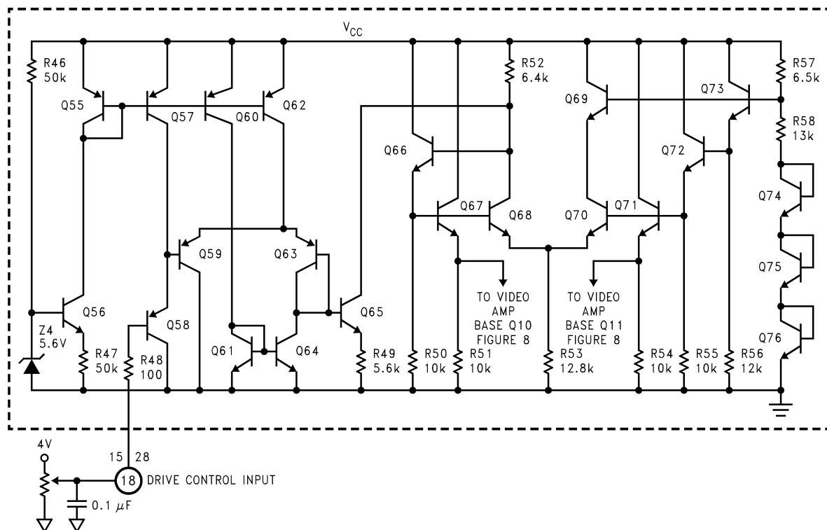
FIGURE 10. Simplified Schematic of LM1208 Drive Control
