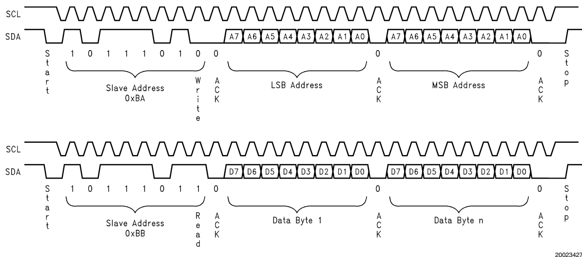
FIGURE 20. I²C Compatible Read Sequence
