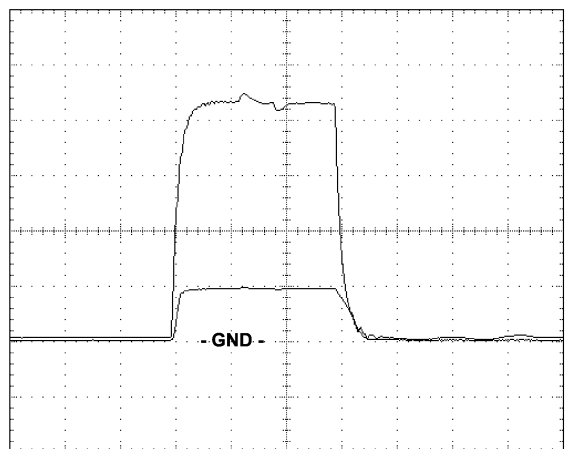
Horizontal: 500 nSec/div Vertical: 1 V/div (both)
