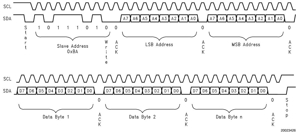
FIGURE 19. I²C Compatible Write Sequence
