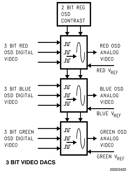
FIGURE 13. Block Diagram of OSD DACs
