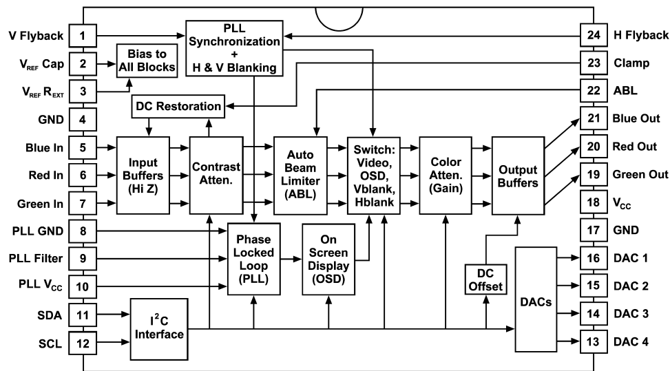
FIGURE 1. Order Number LM1238AAF/NA See NS Package Number N24D
