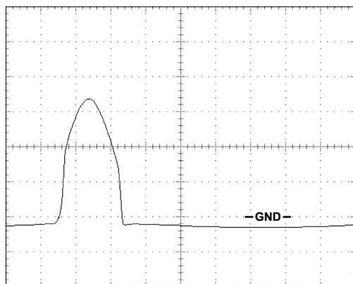
Horizontal: 1 µsec/div Vertical: 500 mV/div
