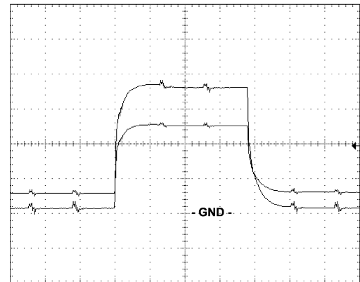
Horizontal: 10 µSec/div Vertical: 1 V/div (both)
