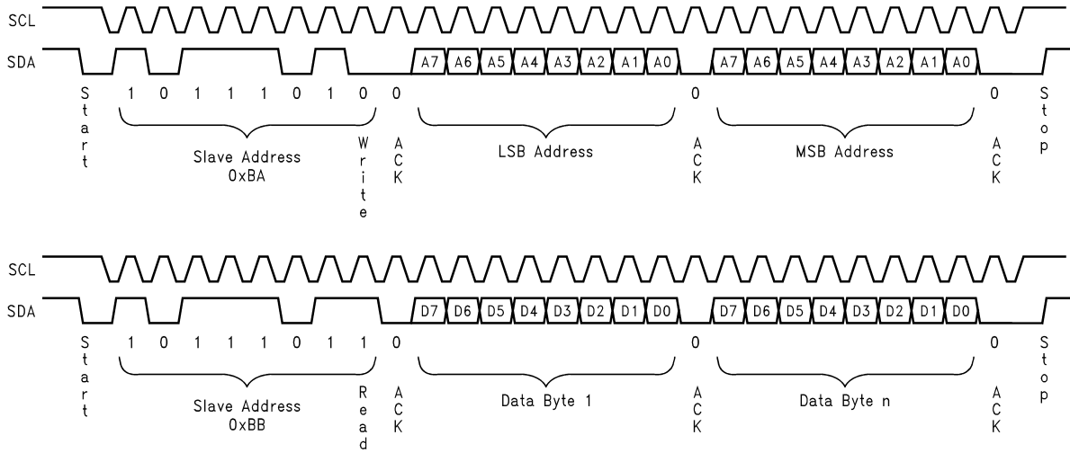
FIGURE 16. I 2 C Compatible Read Sequence
