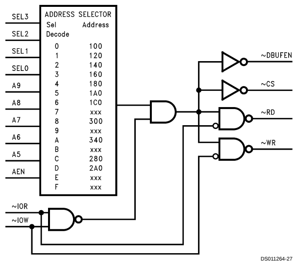
FIGURE 19. GAL Functional Block Diagram
